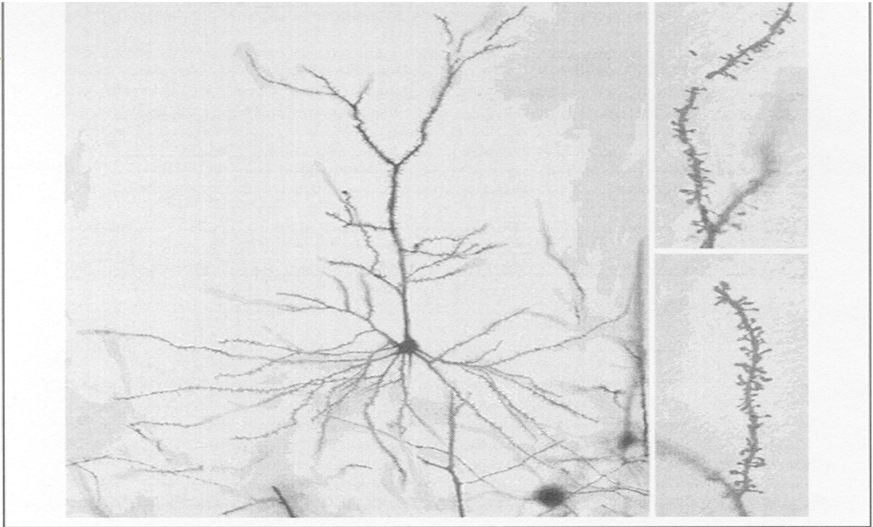
Fig. 1. Photograph of a neuron. In the view on the left, the dendritic field with the extensive dendritic network is visible. On the right are higher-power views of dendritic branches showing the spines, where most synapses are located. If there is an increase in dendritic length, spine density, or both, there are presumed to be more synapses in the neuron.
